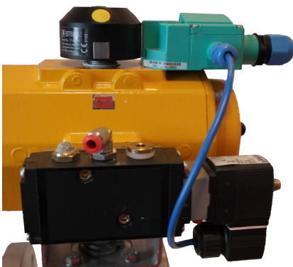
Pneumatic actuator with limit switch pre-wired solenoid
